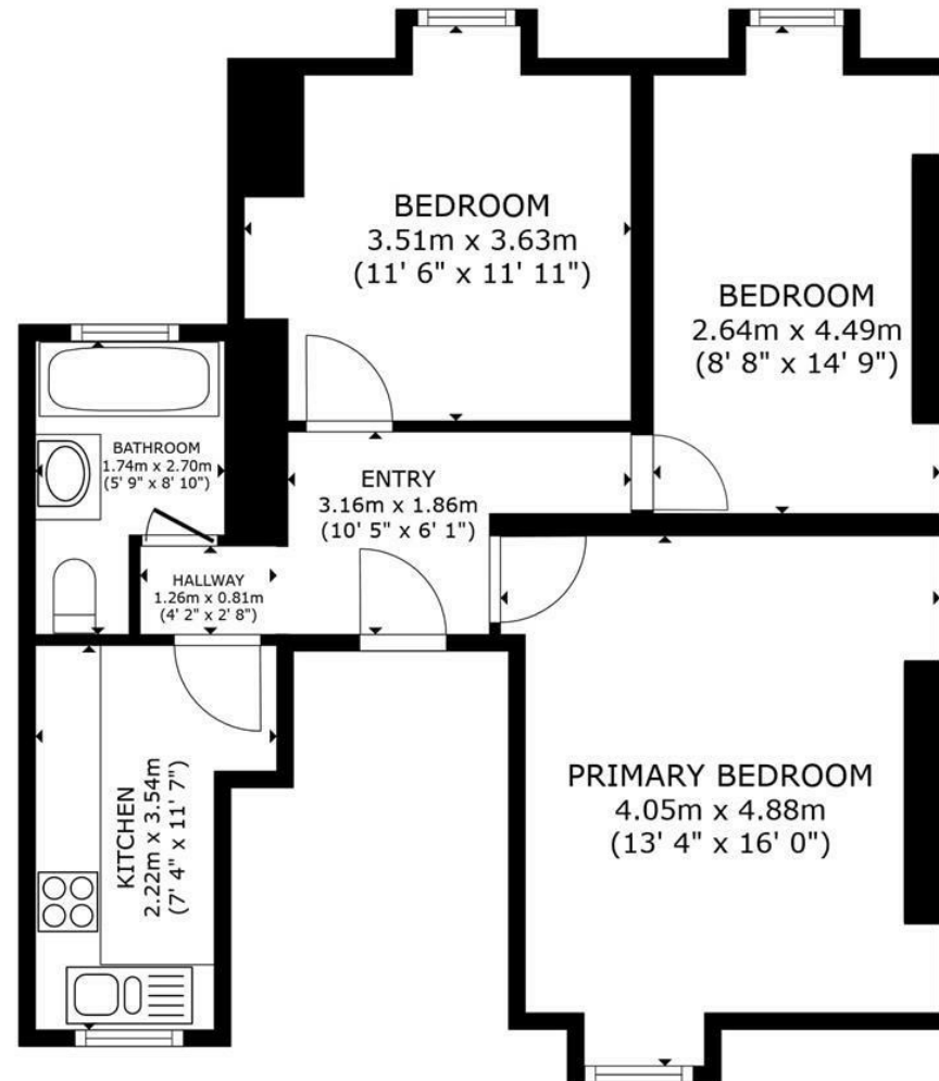
FLOOR PLAN
